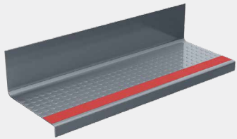
STAIR TREADS WITH RISER FOR THE VISUALLY IMPAIRED (PVR)
