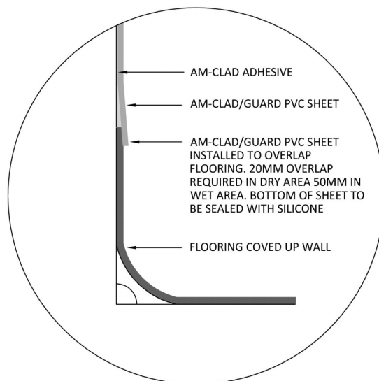
OVERLAP DETAIL (WET AREA)
